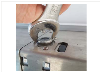
2. Use a 22mm spanner to undo the collar (anti-clockwise to undo)
