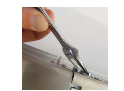
6. Tighten with a ½ turn – DON'T overtighten as the housing material is acetal plastic and easily stripped
