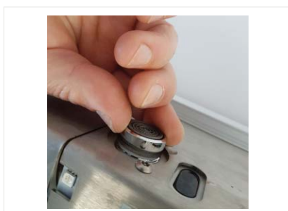
5. Fit the new aerator. MAKE SURE the rubber washer is in place between the aerator and the tap body
