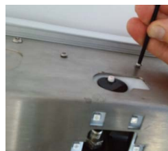
5. Undo the 2 x T20V retaining screws
