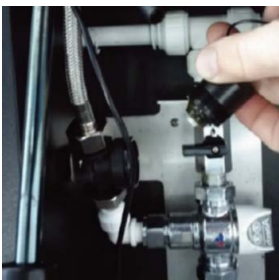
Solenoid clear of body
