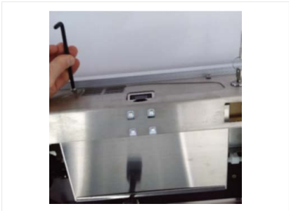
4. Undo the 2nd T30V retaining screw
